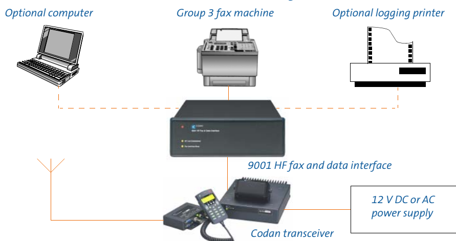
9001 Interconnection diagram
